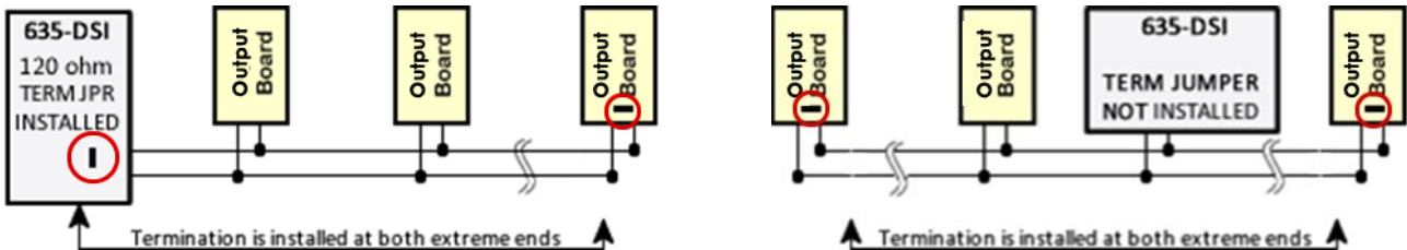
Diagram A: 120 Ω TERM JUMPER INSTALLED ON DSI.
